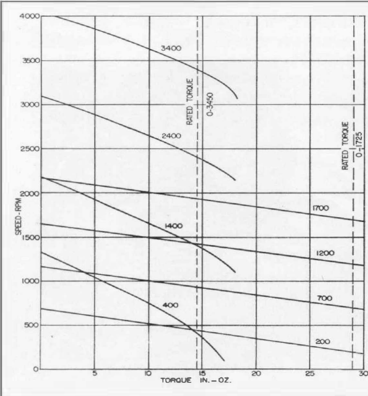
Figure 4. Speed-torque curves for 1/20 h.p. shunt motor with Type 1701-AK Control for the high and low speed ranges.
