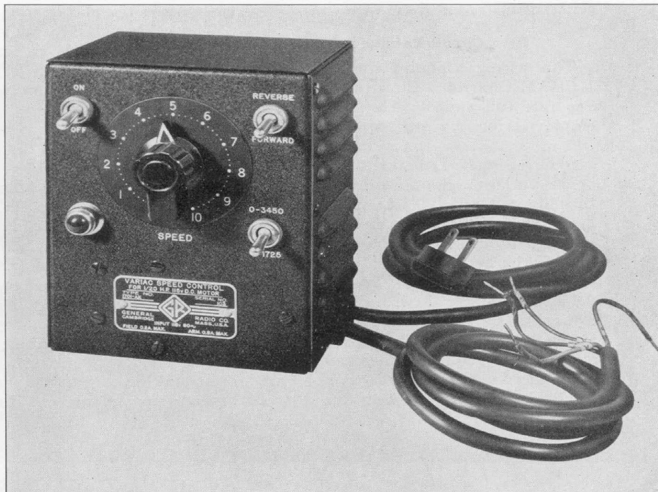
Figure 1. Panel view of the Type 1701-AK Variac Speed Control.
