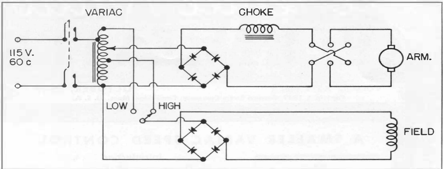
Figure 2. Circuit of Type 1701-AK Speed Control. Circuit of Type 1701-AU is similar but furnishes the field supply at a lower voltage and has only a single speed range.
