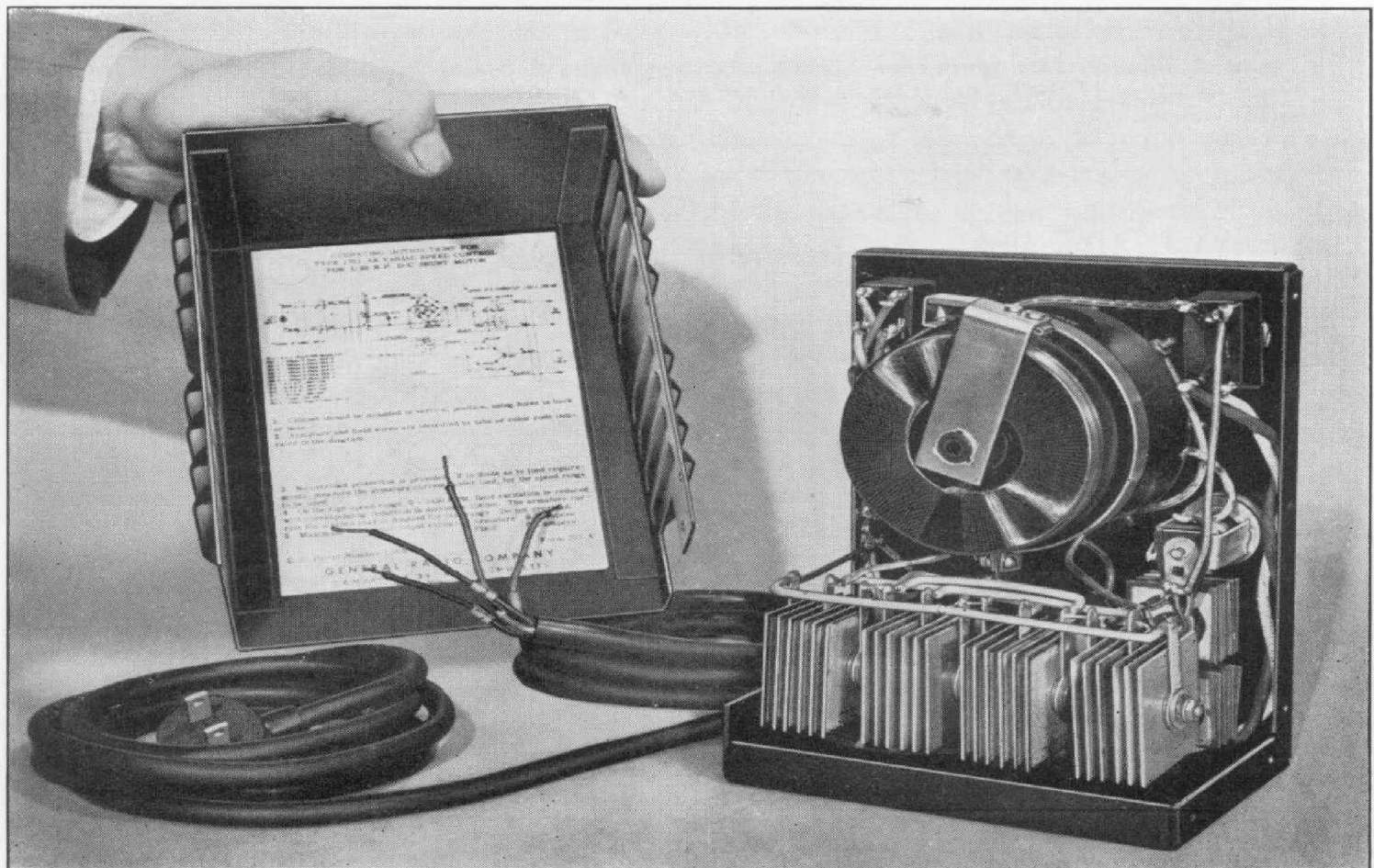
Figure 3. Interior view of control.
