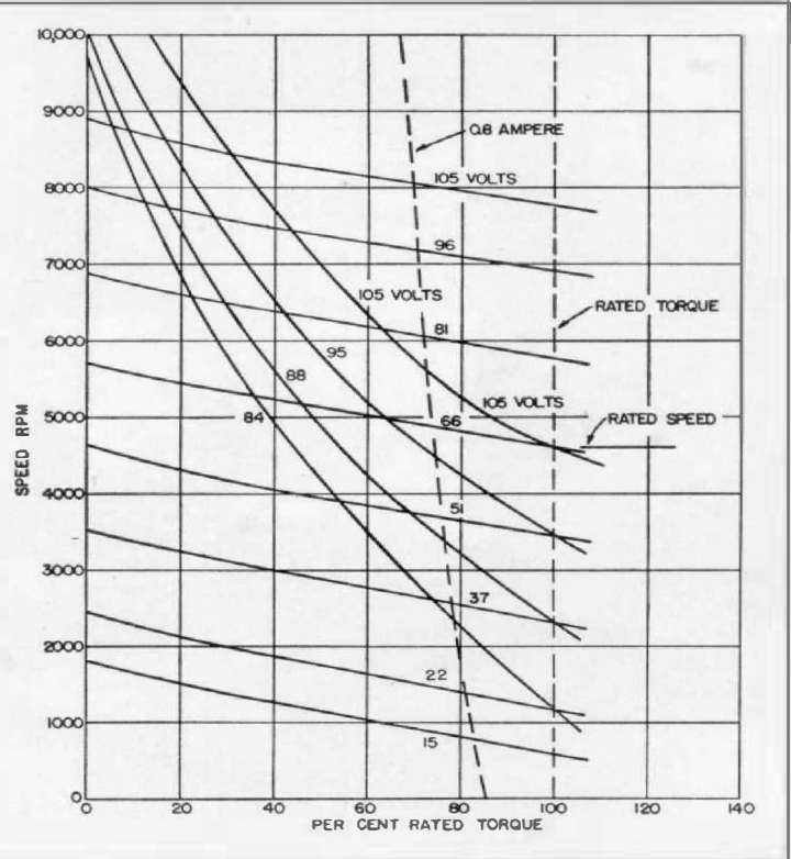
Figure 5. Speed-torque curves for 1/15 h.p. converted universal motor used with Type 1701-AU Control compared with a-c operation of the motor.
